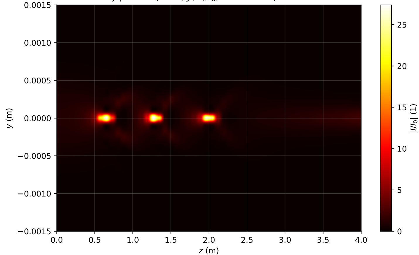
Intensity profile I(x=0, y, z)/I_0 , P_{in}=4.0P_{cr} , artificial time
